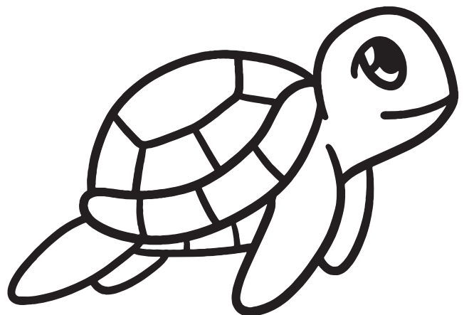
sea turtle
